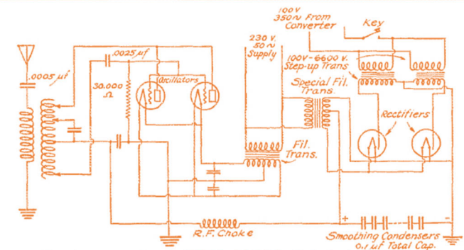
FIG. 3 FINAL TRANSMITTING CIRCUIT AT ENGLISH 5WS
